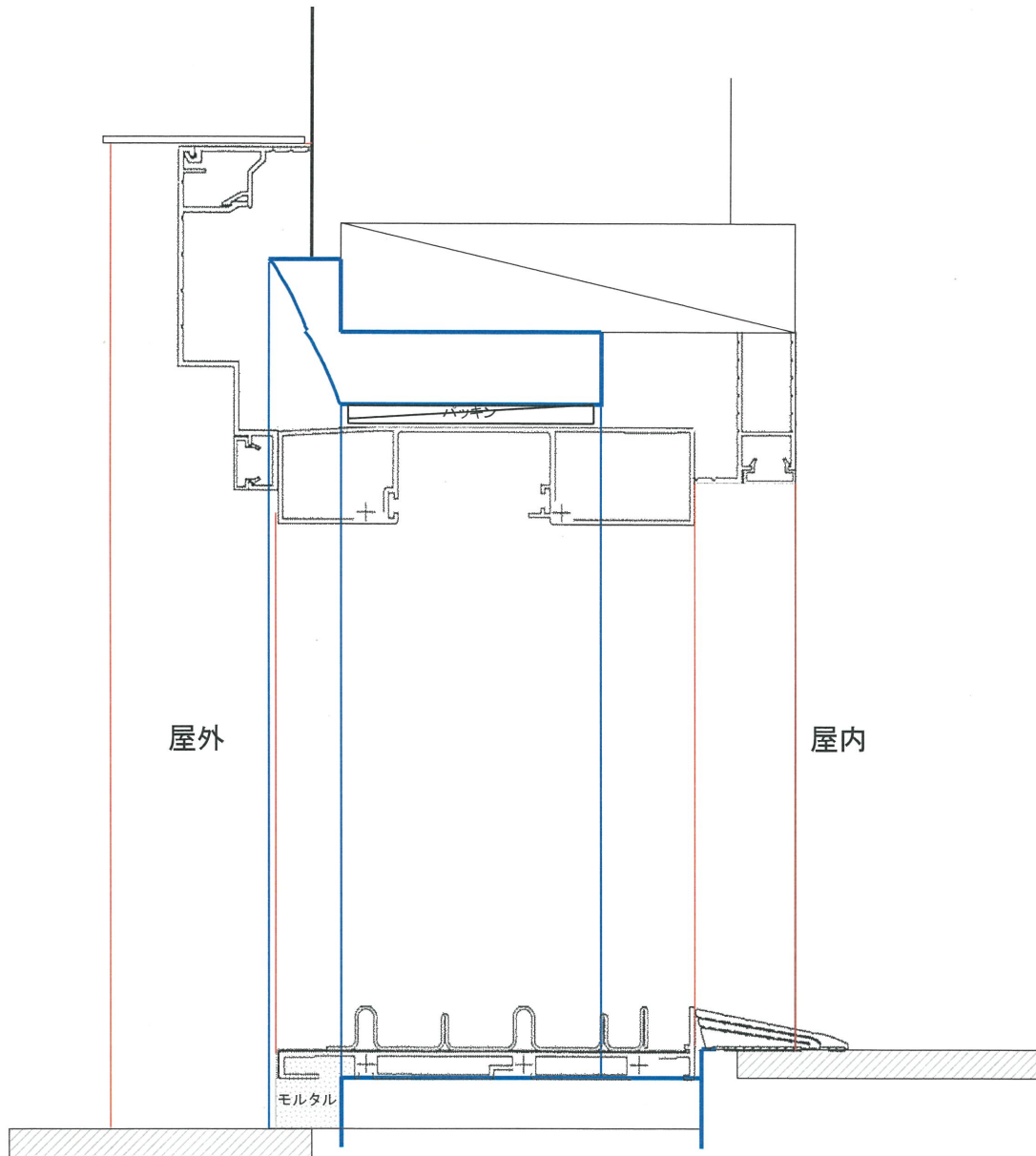
タテ断面1/20
